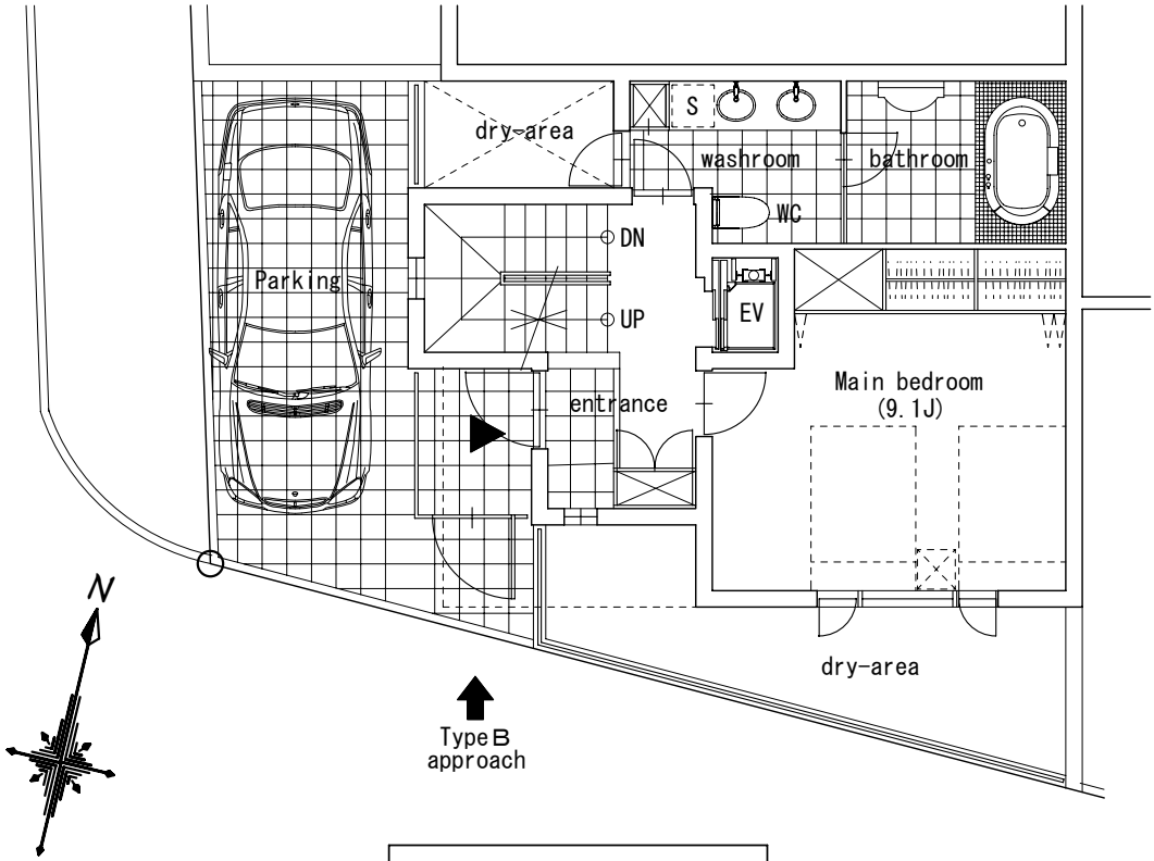
1 floor PLAN S=1/100
